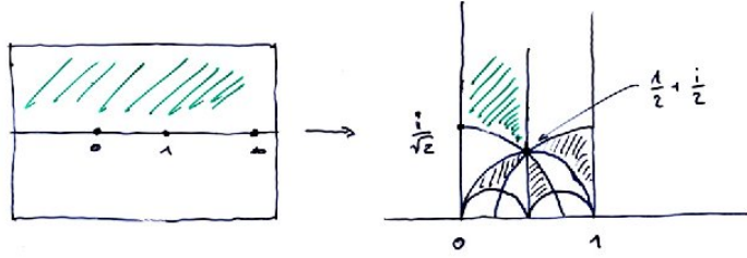
Figure 1.2: Mapping properties of the mirror map \psi in coordinates z = 1/t^4 and p .
