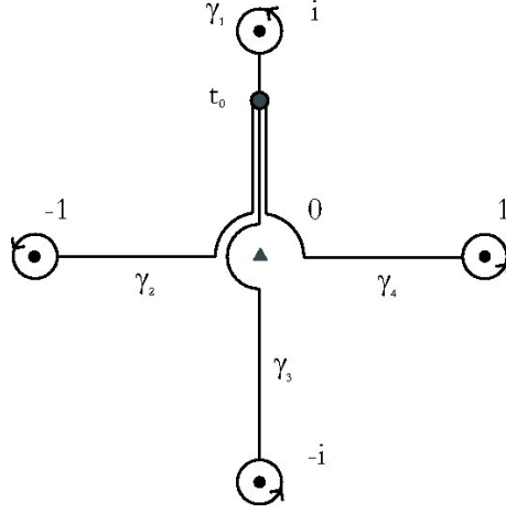
Figure 10.1: Generators of the fundamental group \pi_1(B, t_0) .
